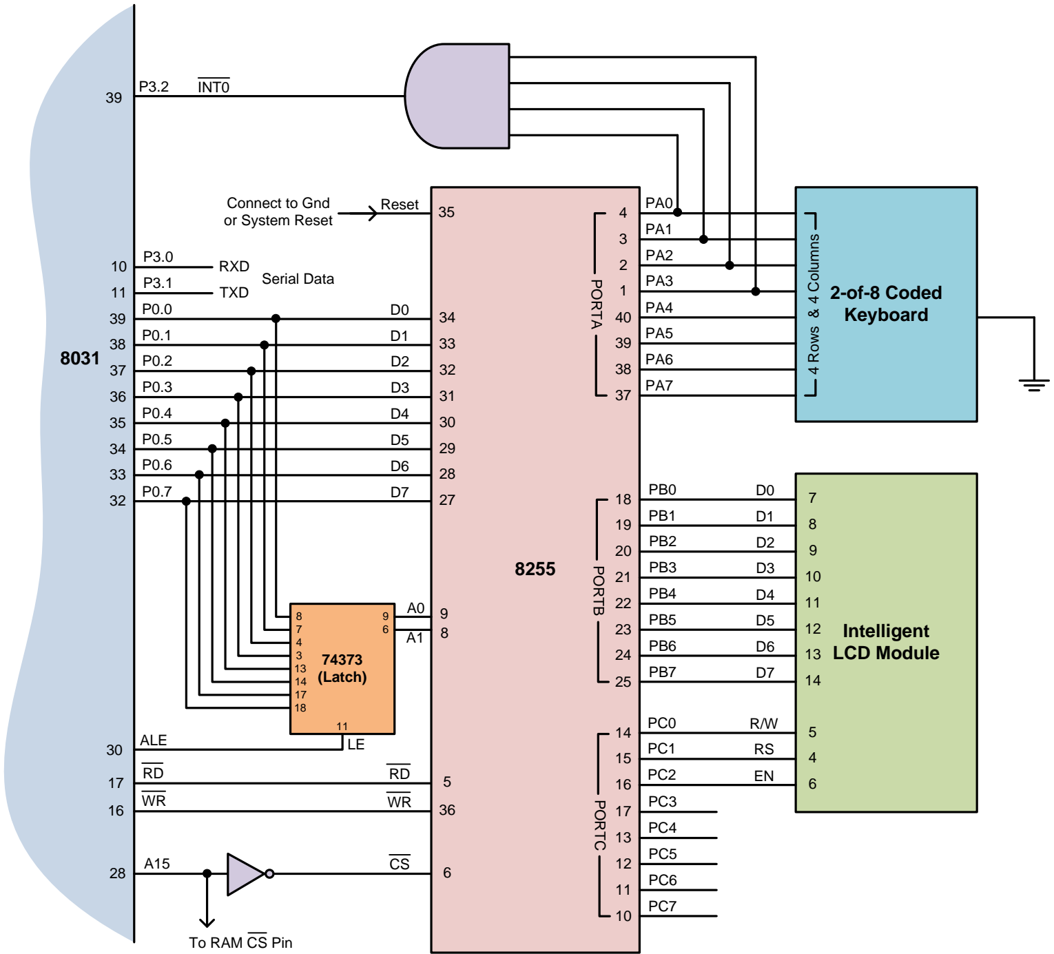
8255 I/O Ports mapped at 8000, 8001 and 8002
